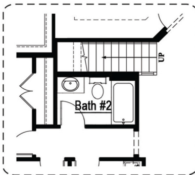
② STAIR LOCATION WITH OPTIONAL SECOND FLOOR
